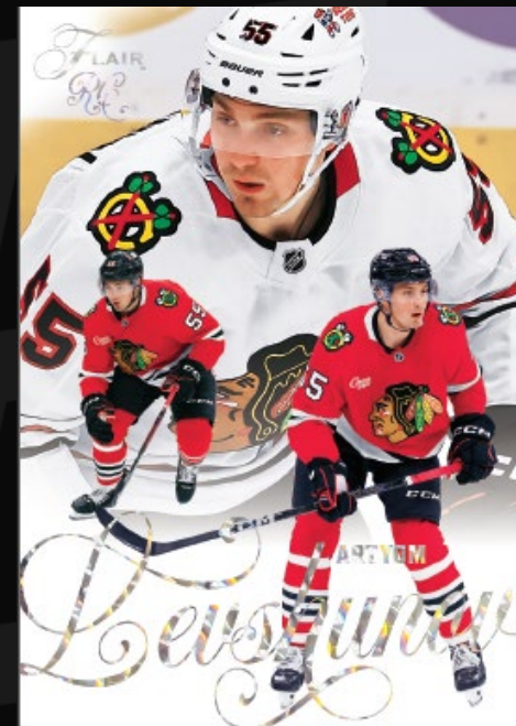
BASE SET Spectrum Parallel
